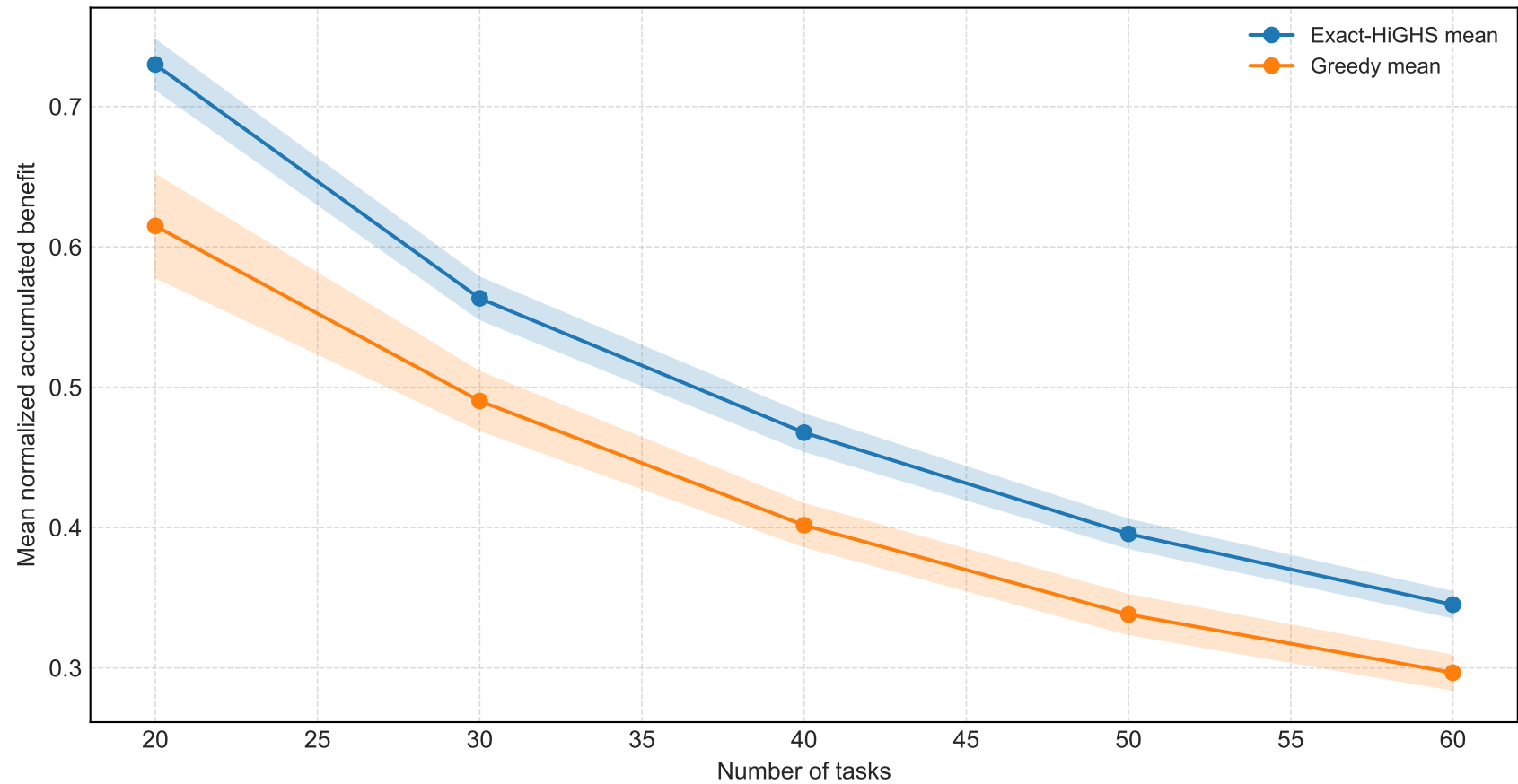
Experiment B: normalized benefit across task counts
